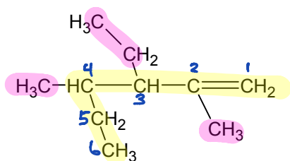
3-ethyl-2,4-dimethyl-1-hexene
