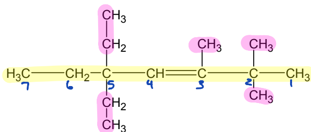
5,5-diethyl-2,2,3-trimethyl-3-heptene
