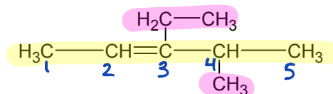
3-ethyl-4-methyl-2-pentene
