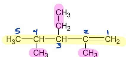
3-ethyl-2,4-dimethyl-1-pentene
