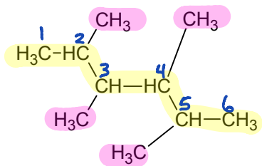
2,3,4,5-tetramethylhexane
