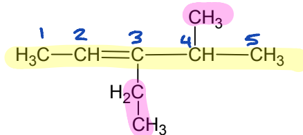
3-ethyl-4-methyl-2-pentene
