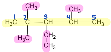
3-ethyl-2,2,4-trimethylpentane
