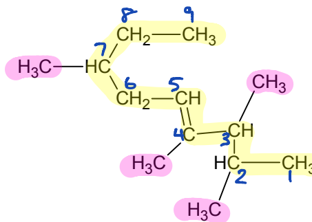
2,3,4,7-tetramethyl-4-nonene
