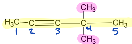
4,4-dimethyl-2-pentyne
