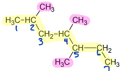
2,4,5-trimethylheptane
