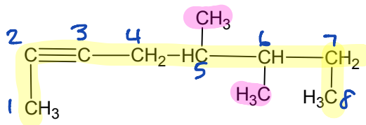
5,6-dimethyl-2-octyne
